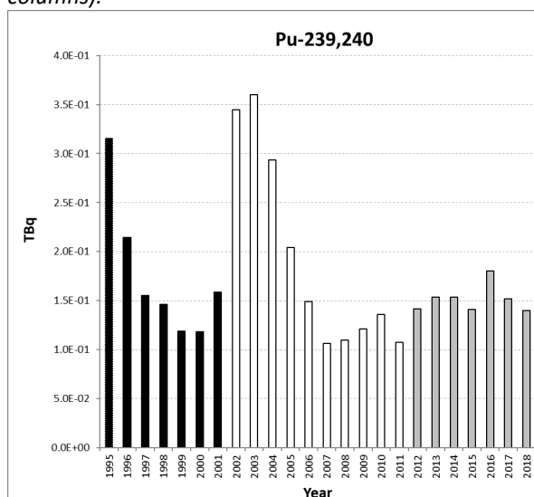
Figure 5.8: Pu-239,240 discharges from the nuclear fuel reprocessing sub-sector for all Contracting Parties for the period 1995 to 2018. Time periods indicated are baseline period (black columns), assessment period (grey columns) and intervening years (white columns).
