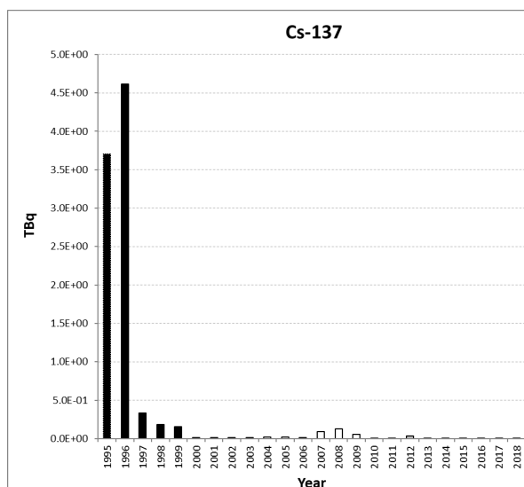
Figure 5.13: Cs-137 discharges from the nuclear research and development sub-sector for all Contracting Parties for the period 1995 to 2018. Time periods indicated are baseline period (black columns), assessment period (grey columns) and intervening years (white columns).
