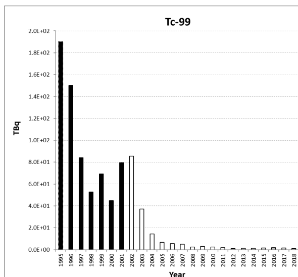
Figure 5.6: Tc-99 discharges from the nuclear fuel reprocessing sub-sector for all Contracting Parties for the period 1995 to 2018. Time periods indicated are baseline period (black columns), assessment period (grey columns) and intervening years (white columns).
