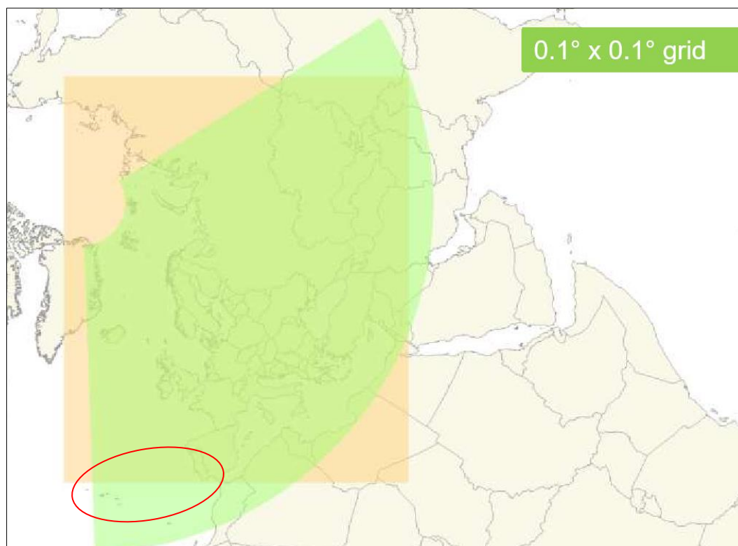
Figure 10.1 – The EMEP grid. Portugal's location.
