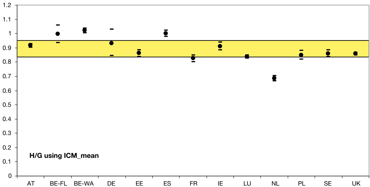
Figure 2.2.16: High / good boundaries proposed by participants in the CB GIG phytobenthos intercalibration exercise. Data points show either the predicted boundary value \pm 95% confidence limits (for those countries with a single H/G boundary value) or the median of all national boundary values, along with the highest and lowest confidence limits of the predictions (for those countries with >1 H/G boundary value). The blue rectangle shows the approximate limits of acceptable boundary values: 0.839 – 0.939.
