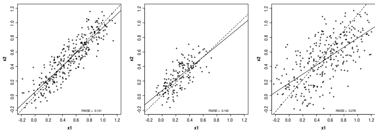
Figure 2.2.10: Model I and Model II regressions for 3 hypothetical datasets. The left and central plot have the same amount of error and the same RMSE of 0.14, even though they cover different ranges (their product moment correlations are very different – 0.9 for left plot, 0.64 for centre). The right plot shows data with the same trend but double the error. In this case the RMSE = 0.28, r = 0.66 . The central figure has a clearly better agreement between x_1 and x_2 than the right-hand one but their correlations are very similar.
