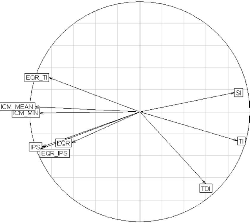
Figure 2.2.12: Factorial map of a correlation circle, based on PCA presented in Fig.2.2.11.
