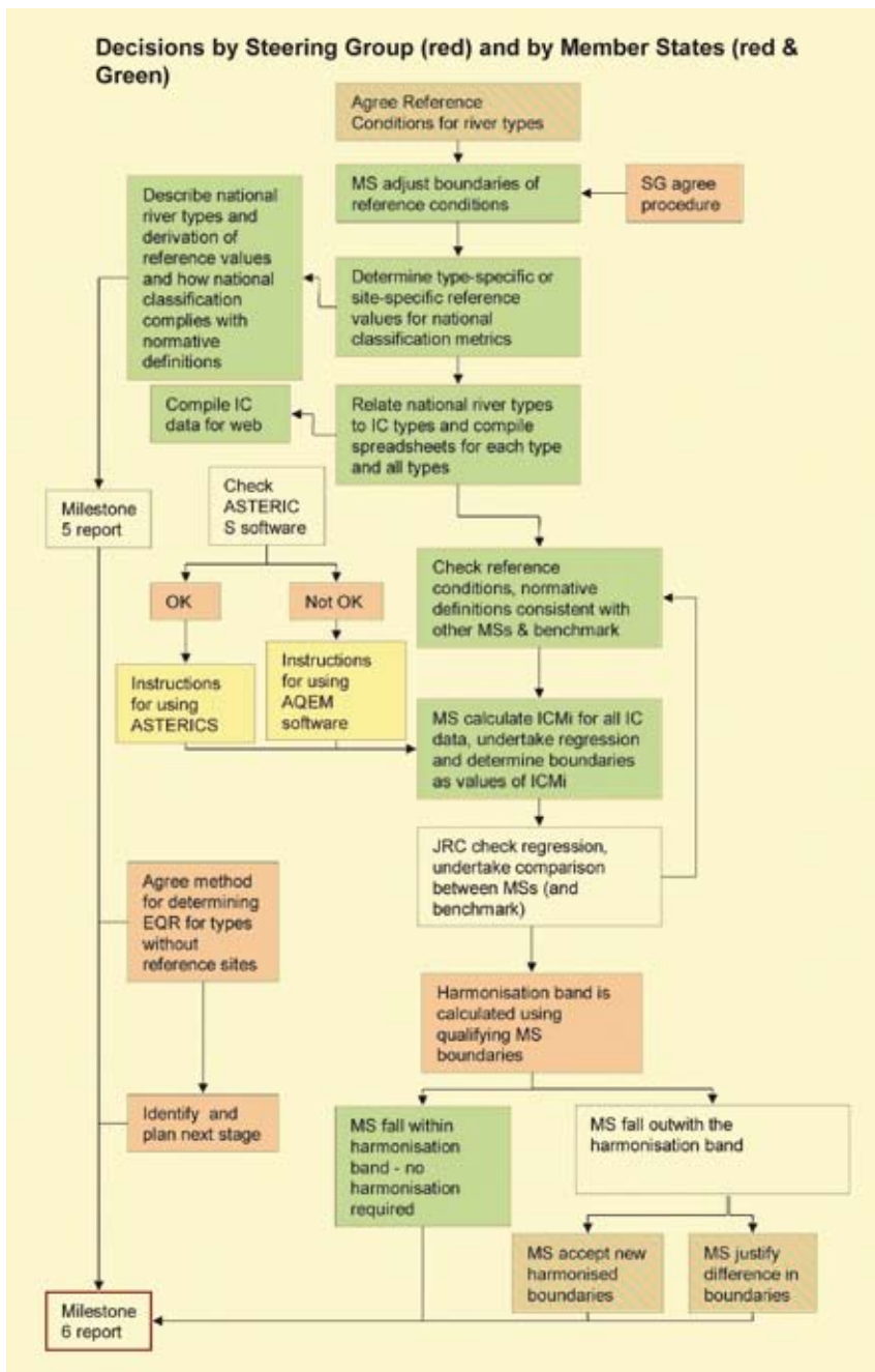
Figure 2.1.1: Flow diagram to demonstrate the CB GIG rivers comparison and harmonisation procedure, and the roles of the Steering Group and the Member States in the process (further explanations see text).
