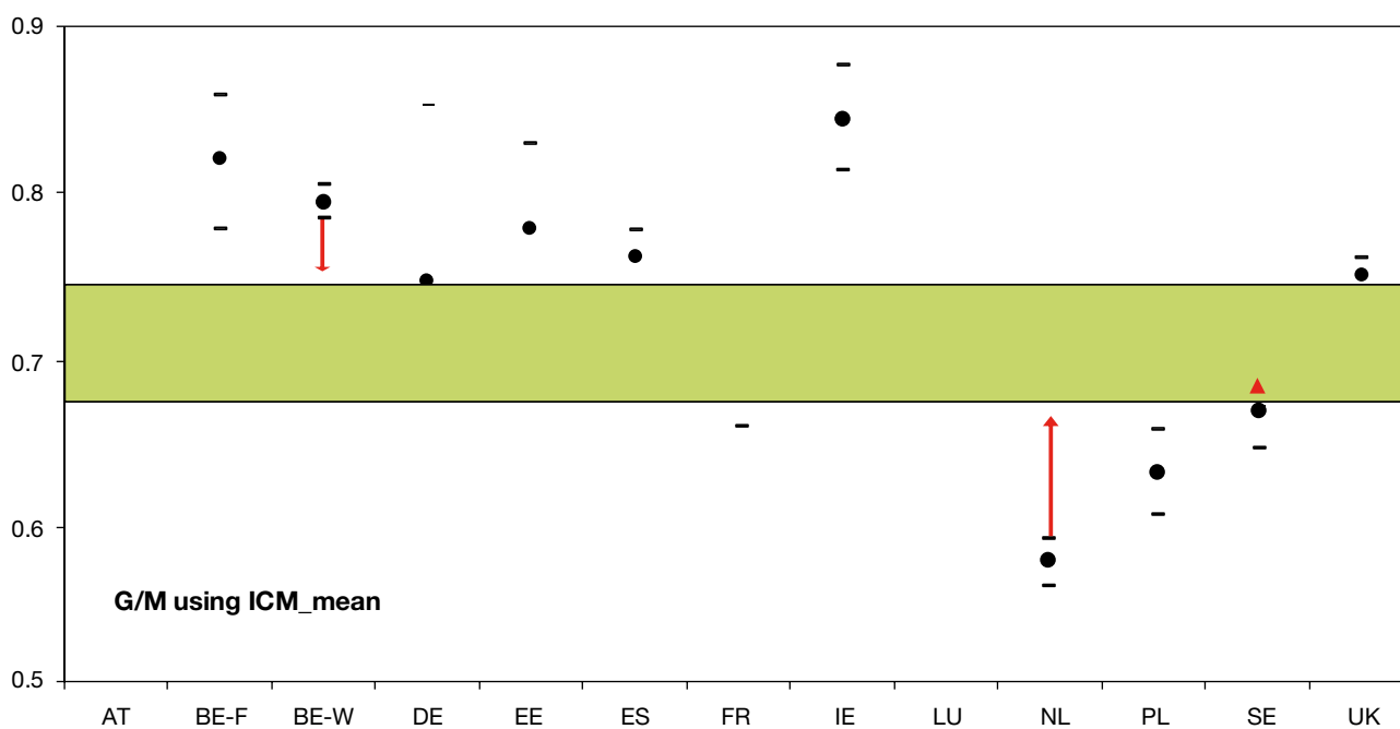
Figure 6.4: EQR_ICM values for the Good / moderate boundary following the incorporation of changes (red arrows) made during the harmonisation stage of the Intercalibration exercise.
