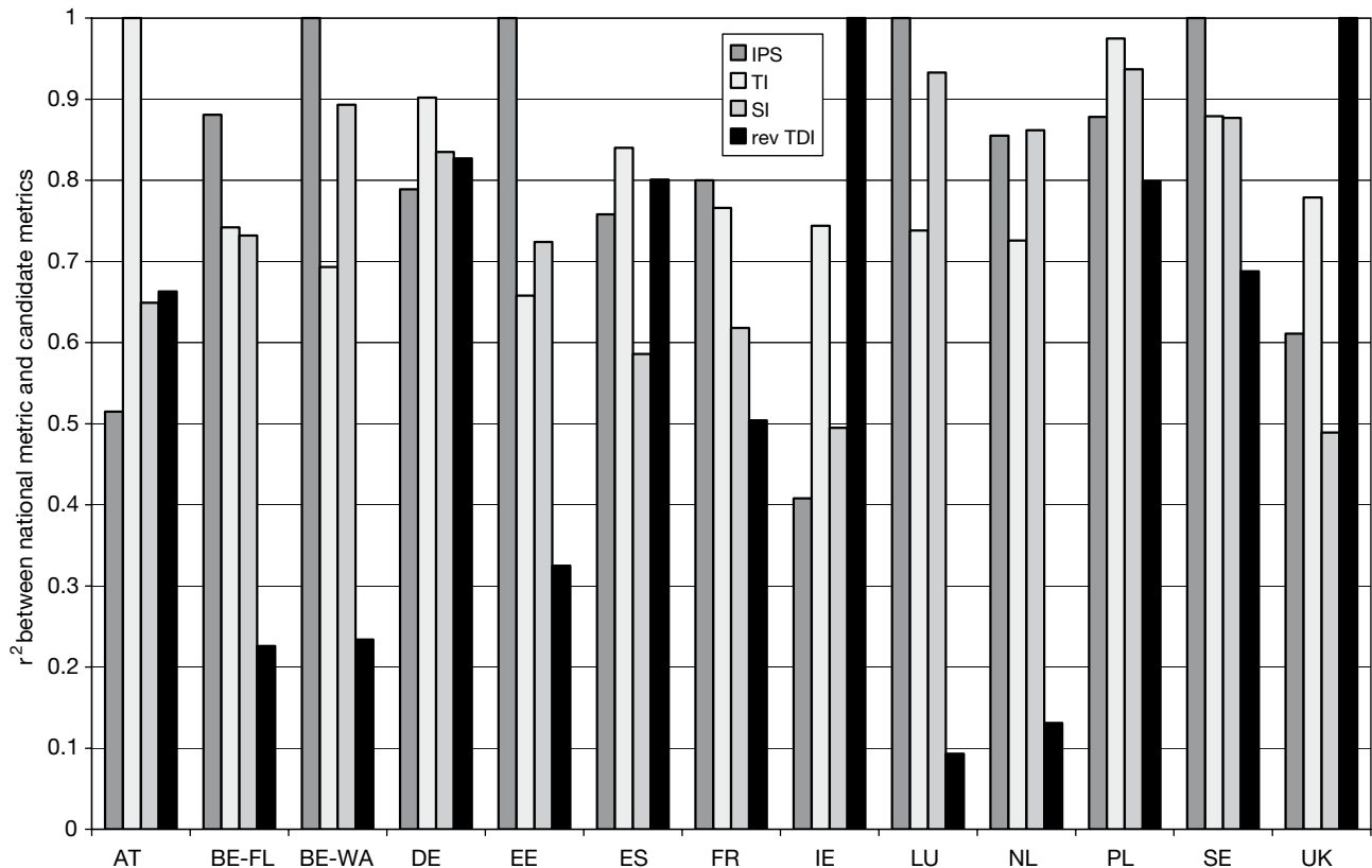
Figure 2.2.8: Performance of four candidate ICMs against national metrics expressed in terms of the coefficient of determination, r^2 . Where a candidate ICM is also a national metric, r^2 = 1 .
