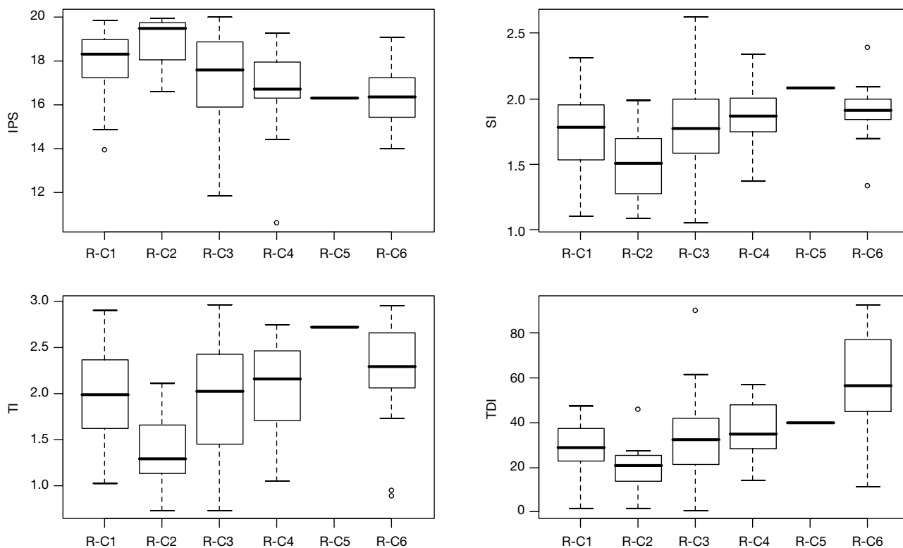
Figure 2.2.1: Variation in values of candidate metrics between intercalibration (IC) types. Differences between IC types are significant at p < 0.001 for IPS, TI and TDI and at p < 0.01 for SI.
