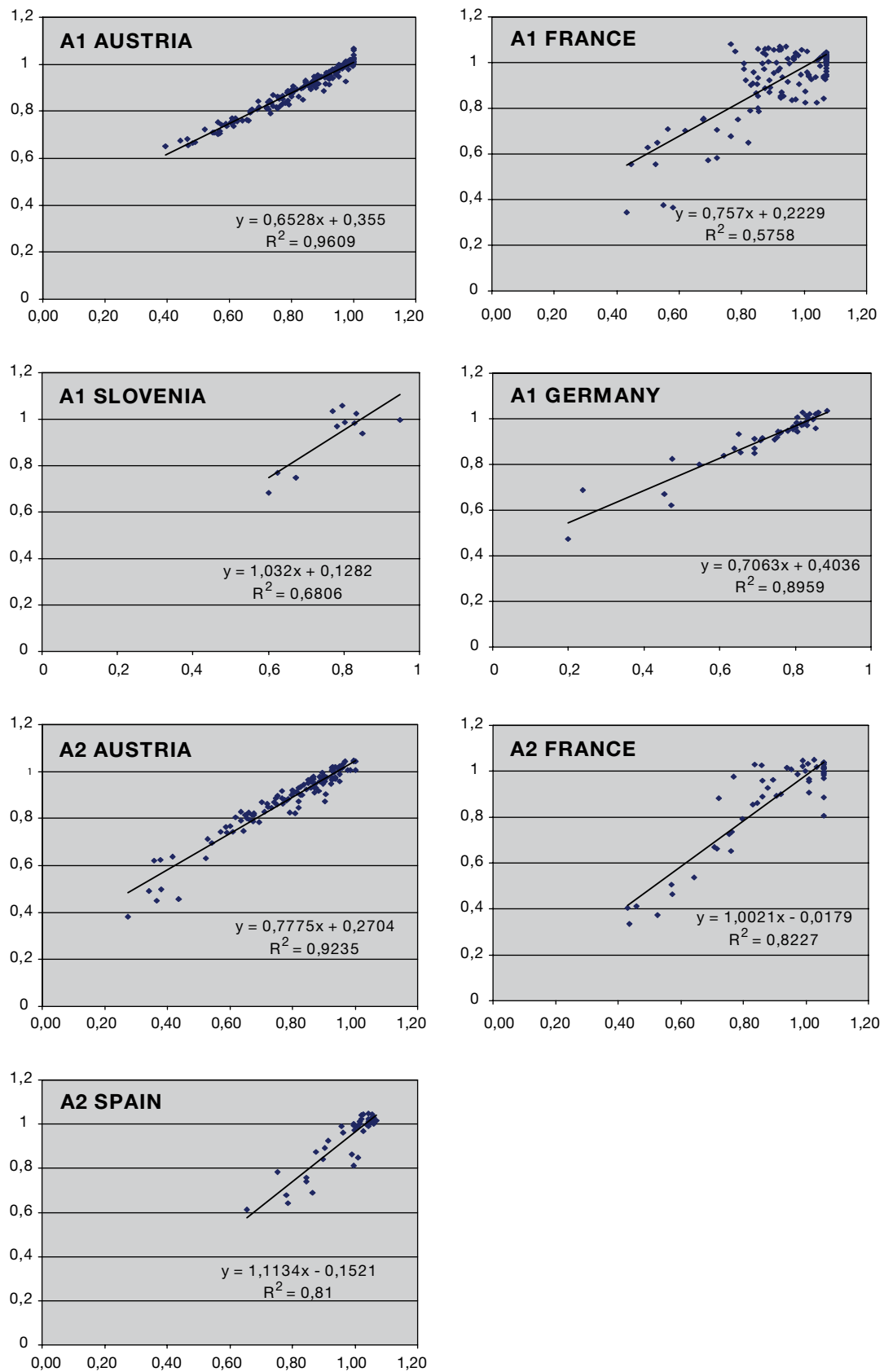
Figure 2.3.1: Regression: x-axis = national method and y-axis = ICM
