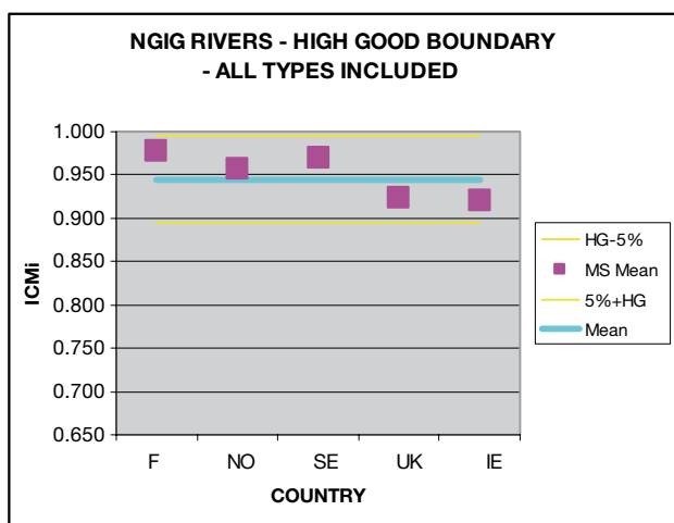
Figure 2.2.1: Results of the comparison showing MS EQR_ICMi values for the H/G boundary. ‘Band’ represents the GIG H/G boundary value. The ‘harmonisation band’ represents \pm 0.05 of the ICMi_EQR scale around the GIG boundary value.
