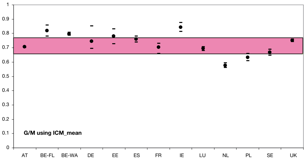
Figure 2.2.17: Good / moderate boundaries proposed by participants in the CB GIG phytobenthos intercalibration exercise. Data points show either the predicted boundary value \pm 95% confidence limits (for those countries with a single G/M boundary value) or the median of all national boundary values, along with the highest and lowest confidence limits of the predictions (for those countries with >1 G/M boundary value). The green rectangle shows the approximate limits of acceptable boundary values: 0.654 – 0.754.
