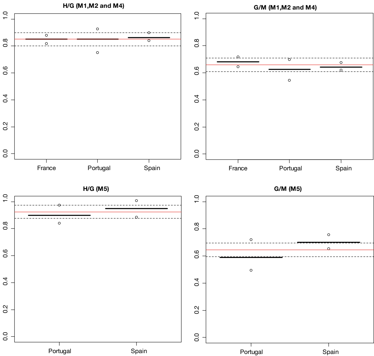
Figure 2.4.4: High/Good and Good /Moderate boundaries proposed by participants in the Med GIG phytobenthos intercalibration exercise, and acceptability bands (dashed line).
