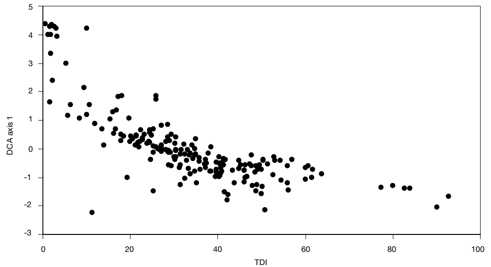
Figure 2.2.3: Relationship between trophic diatom index (TDI) and the first axis of the DCA illustrated in Fig. 2.2.2.
