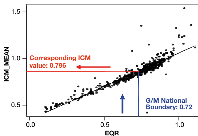
Figure 2.2.14: Conversion of the Good/Moderate national boundary value for a hypothetical national dataset into an ICM value using the regression shown in Fig. 2.2.13.
