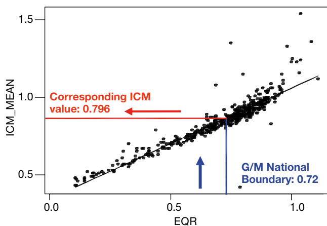
Figure 2.1.1: Conversion of the Good/Moderate national boundary value for a hypothetical national dataset into an ICM value using the regression formula: ICM = a + b (national metric as EQR).
