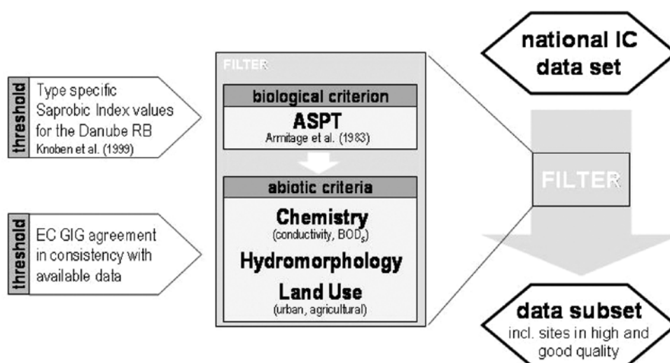
Figure 2.5.1: Harmonised definitions of quality criteria/thresholds for sites in high and good ecological status
