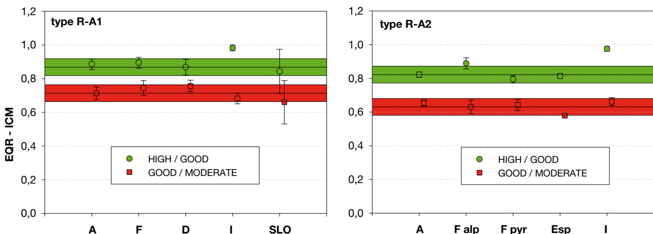
Figure 2.3.1: Boundary values high/good and good/moderate at the ICMi scale +/- 95% confidence limits. Values are taken from the regression between the EQR values of the national method and the EQR values from the ICMi method. The band indicates an „acceptable range of variation“and consist of the median of the boundary values of all member states +/- ¼ of the the median status class width of all member states.
