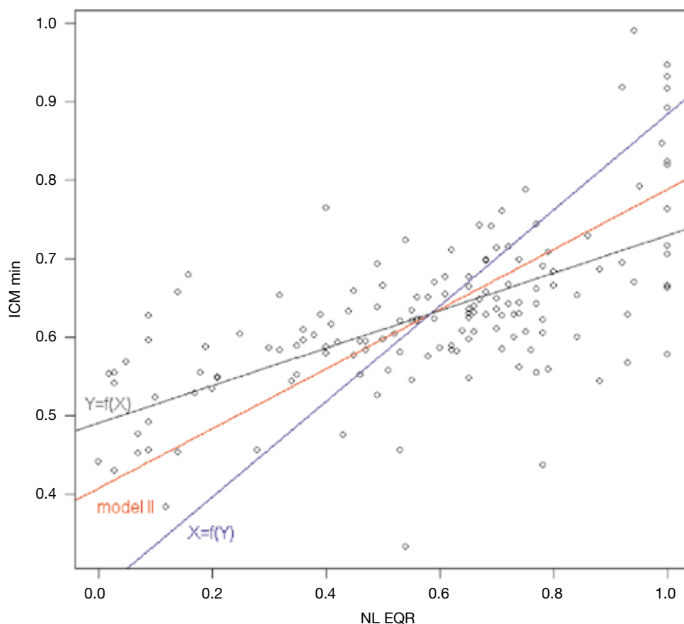
Figure 2.2.9: Model I and model II regression equations for the Dutch dataset used in the phyto­benthos intercalibration exercise. In model I regression, the sum of vertical squared deviations is minimised when regressing Y on X; the same thing occurs horizontally when regressing X on Y. In model II regression, the sum of squared Euclidian distances to the regression line is minimised. Fitted results are the same from X to Y as well as from Y to X with a model II regression; this is not the case for model I (generally).
