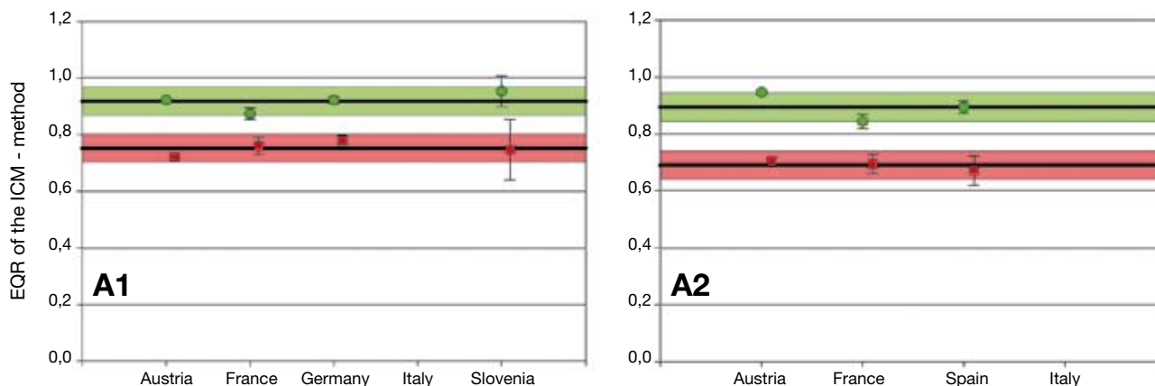
Figure 2.3.2: Comparison of the national boundary values when converted into ICM – values (+/- 95% CL). Green: High/Good boundary, Red: Good/Moderate boundary. The bands show the average boundary values (bold line) +/- 0.05.
