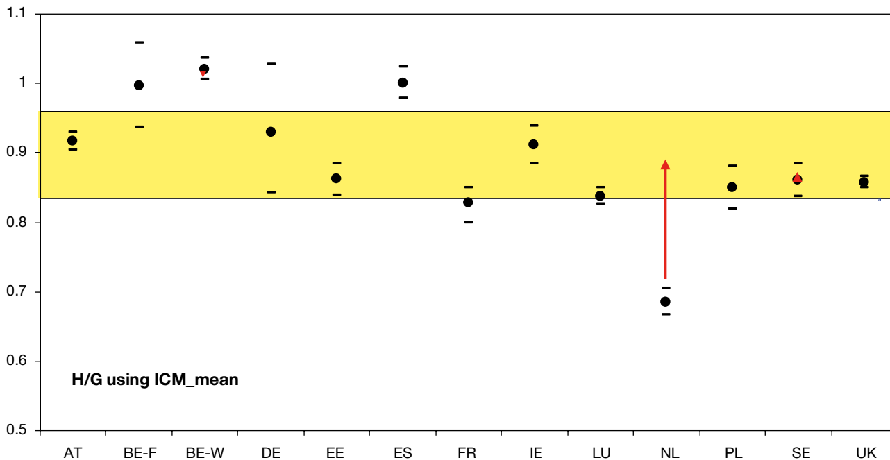
Figure 6.3: MS EQR_ICM values for the High / Good boundary following the incorporation of changes (red arrows) made during the harmonisation stage of the Intercalibration exercise.
