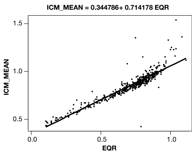
Figure 2.2.13: Relationship between EQR of a national metric and the ICM for a hypothetical national dataset.
