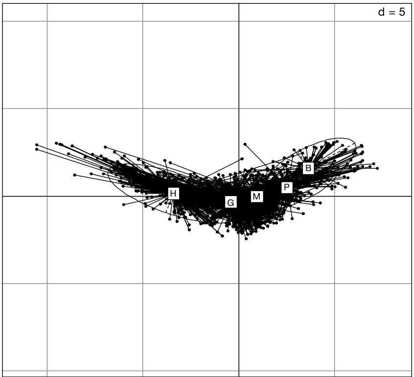
Figure 2.2.11: Principal components analysis (PCA) of index values for all samples in the CB GIG intercalibration database (H: High, G: Good, M: Moderate, P: Poor, B: Bad).
