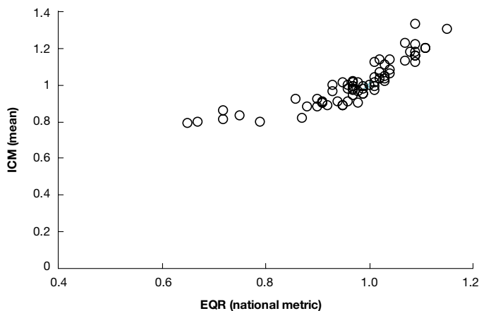
Figure 2.2.15: Relationship between national metrics of Estonia and the intercalibration metric (ICM mean) (adjusted R^2 and RMSE for a second-order polynomial equation are 0.061 and 0.828).
