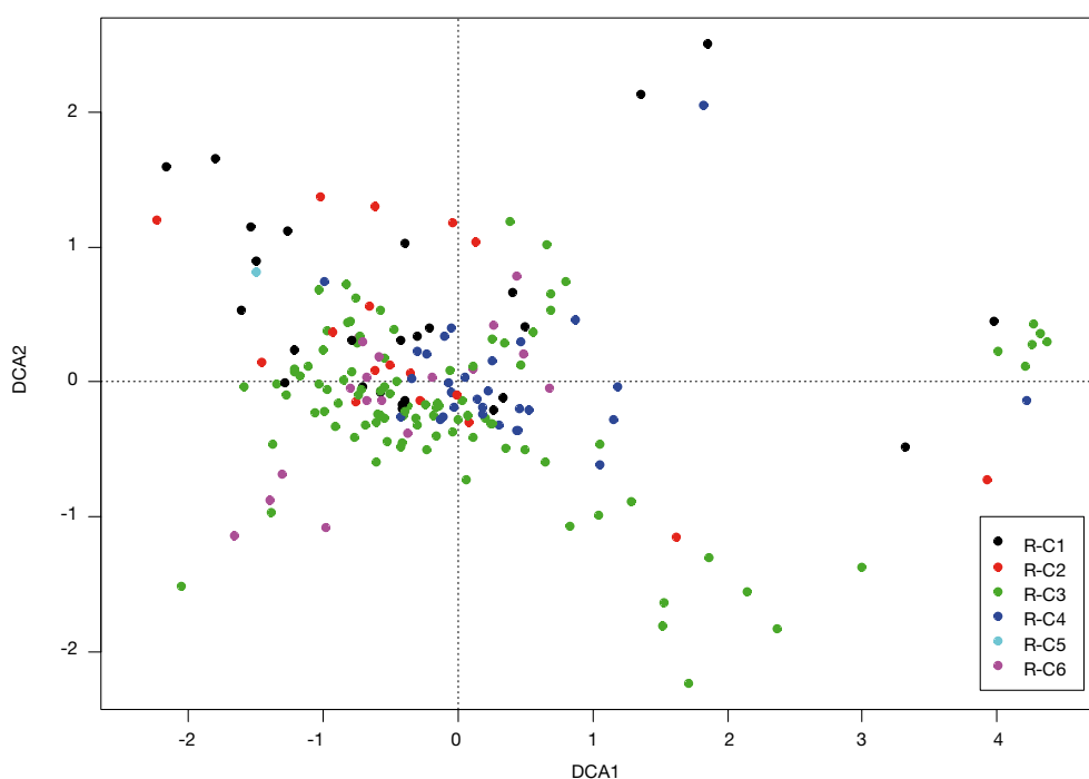
Figure 2.2.2: Detrended correspondence analysis (DCA) of 190 phytobenthos reference samples from Central Baltic GIG, plotted by intercalibration type.
