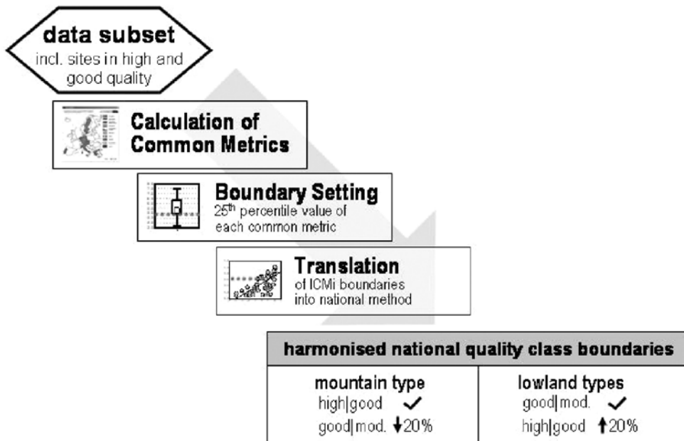
Figure 2.5.2: Class boundary setting using ICMi.
