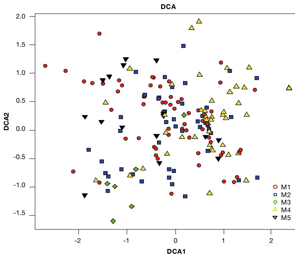
Figure 2.4.2: Detrended Correspondence Analysis (DCA), plotted by intercalibration type.
