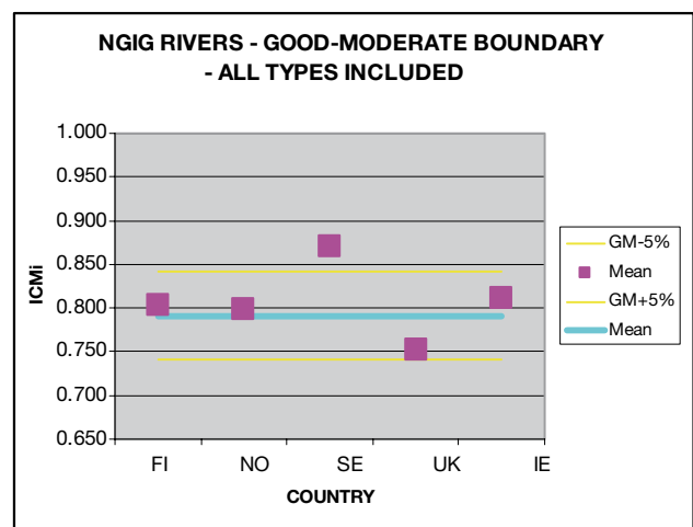
Figure 2.2.2: Results of the comparison showing MS EQR_ICMi values for the G/M boundary. ‘Band’ represents the GIG H/G boundary value. The ‘harmonisation band’ represents \pm 0.05 of the ICMi_EQR scale around the GIG boundary value.
