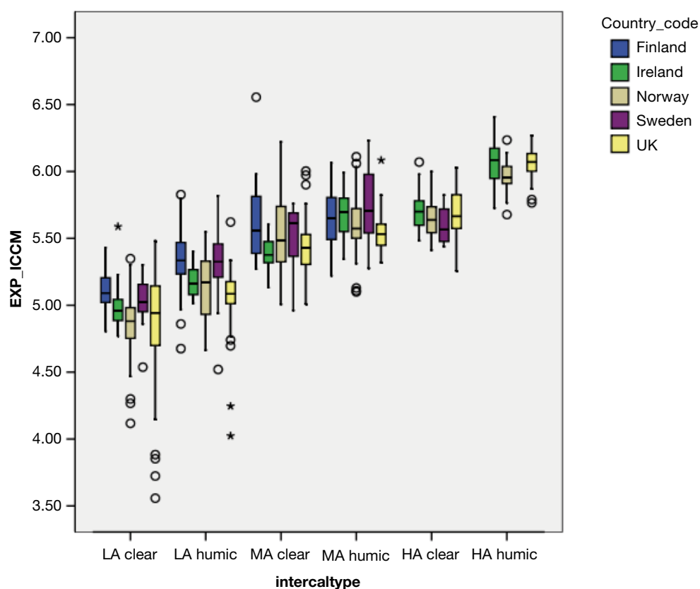
Figure 2.3.4.6a: Range of modelled reference ICCM values for lakes in N-GIG common data set (EXP_ICCM – expected ICCM value).
