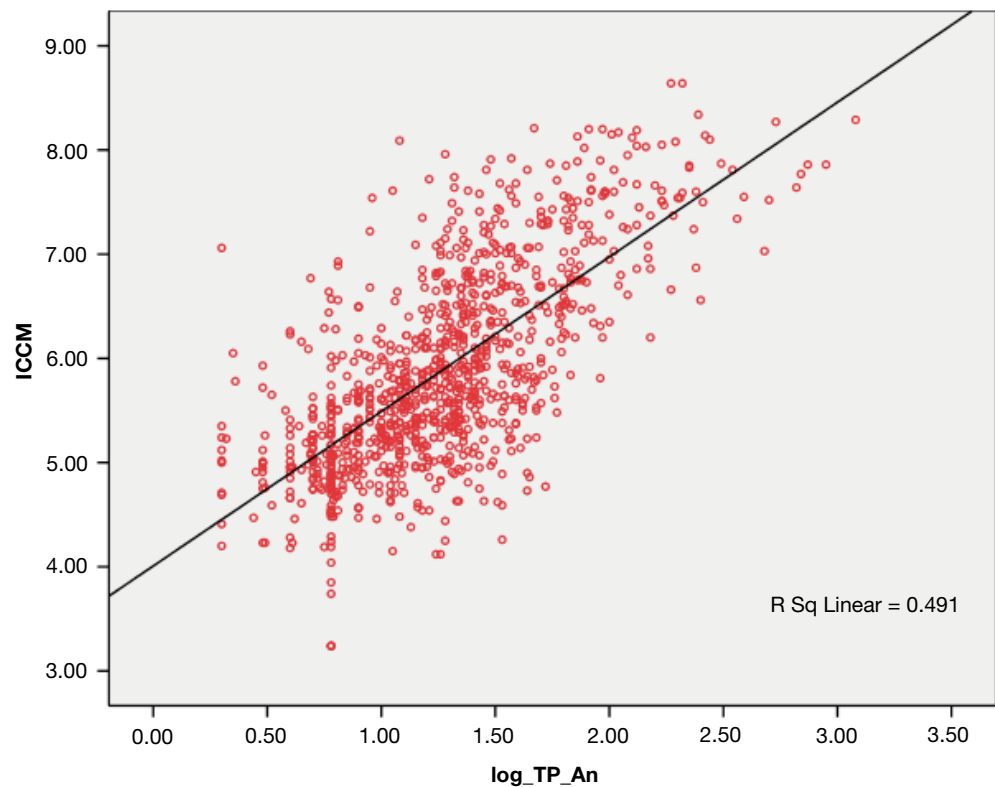
Figure 2.3.6.1b: Relationship between lake ICCM and mean TP concentrations in the global N-GIG dataset (n=1074 surveys).
