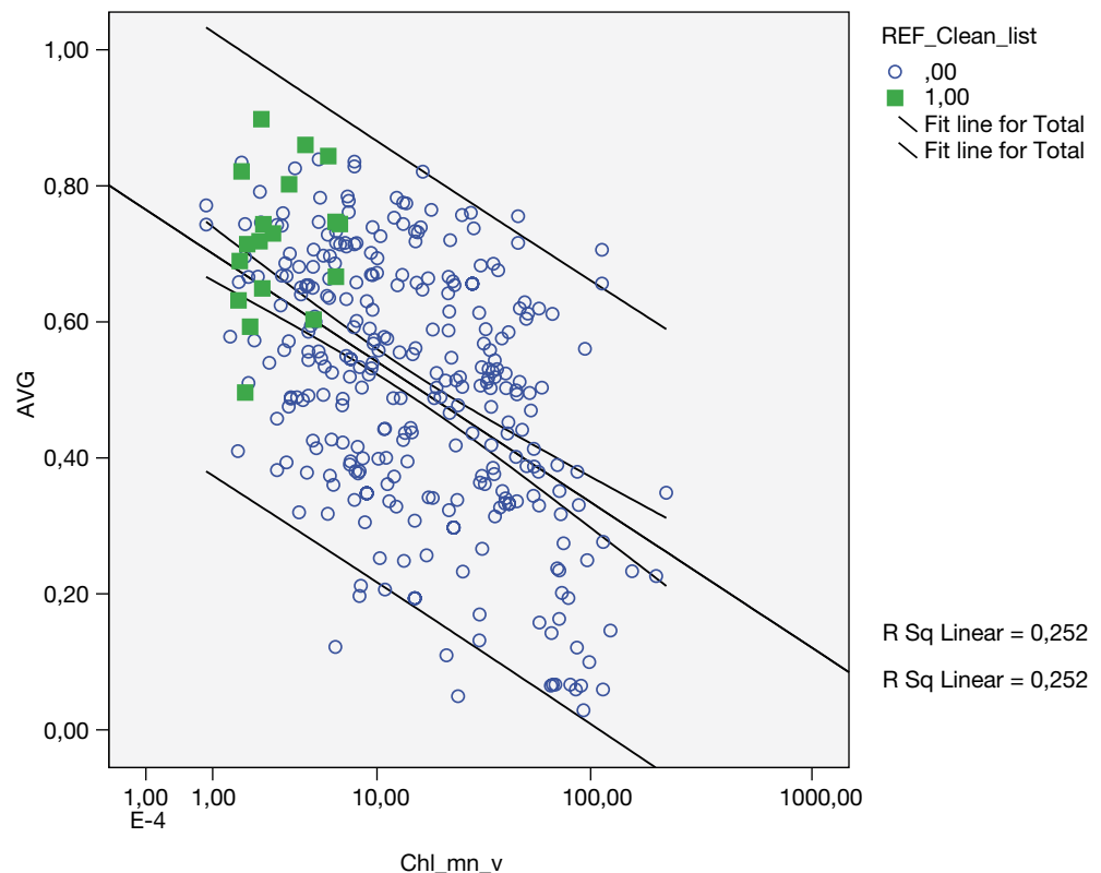
Figure 2.2.4b: Averaged EQR of national assessments (AVG) of the macrophyte composition of sites in the common data base in relation to the mean concentration chlorophyll- a (Chl_mn_v in \mu\text{g l}^{-1} ). The reference sites are presented as squares (L-CB1 and L-CB2 combined). Individual 90% confidence and 95% confidence limits of the regression are shown.
