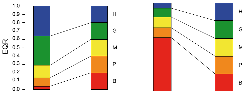
Figure 2.1.6a: Scheme of transforming the EQR values to normalised EQR values with linear scale and equal class widths. Left: total biovolume, right: Brettum index (both for L-AL3).
