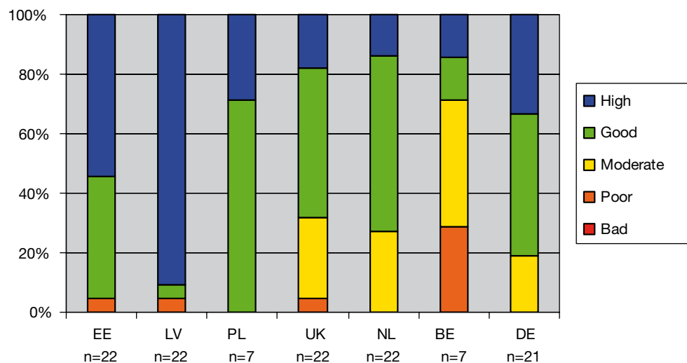
Figure 2.2.4.a: Application of national assessment methods to the common set of reference sites. Note: the Polish and Belgian methods could only be applied to seven sites.
